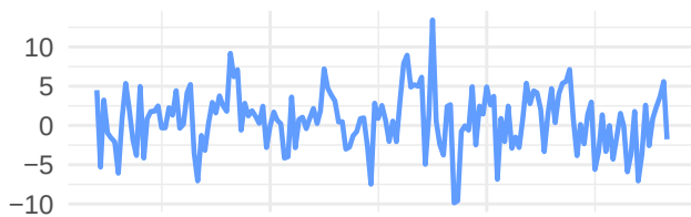
y_us_gap
