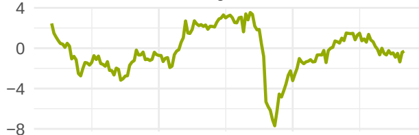
pi_core_gap
