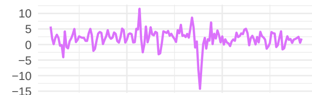
pi_us
